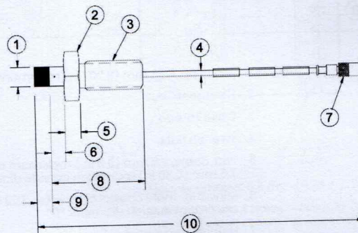
Figure 4: Installed Connector Protectors
